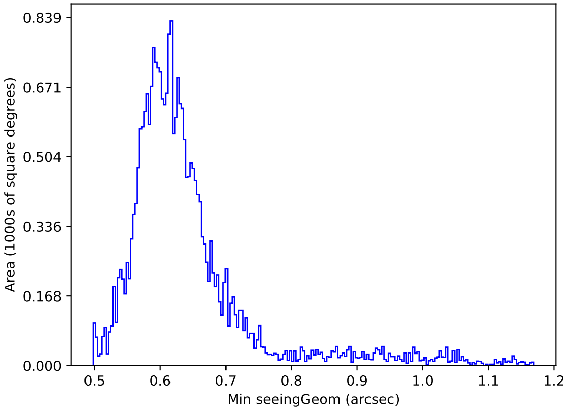
ddf_acor_sf25_lsf30_lsr10_v3.4_10yrs Yr 1 r band: Min seeingGeom
