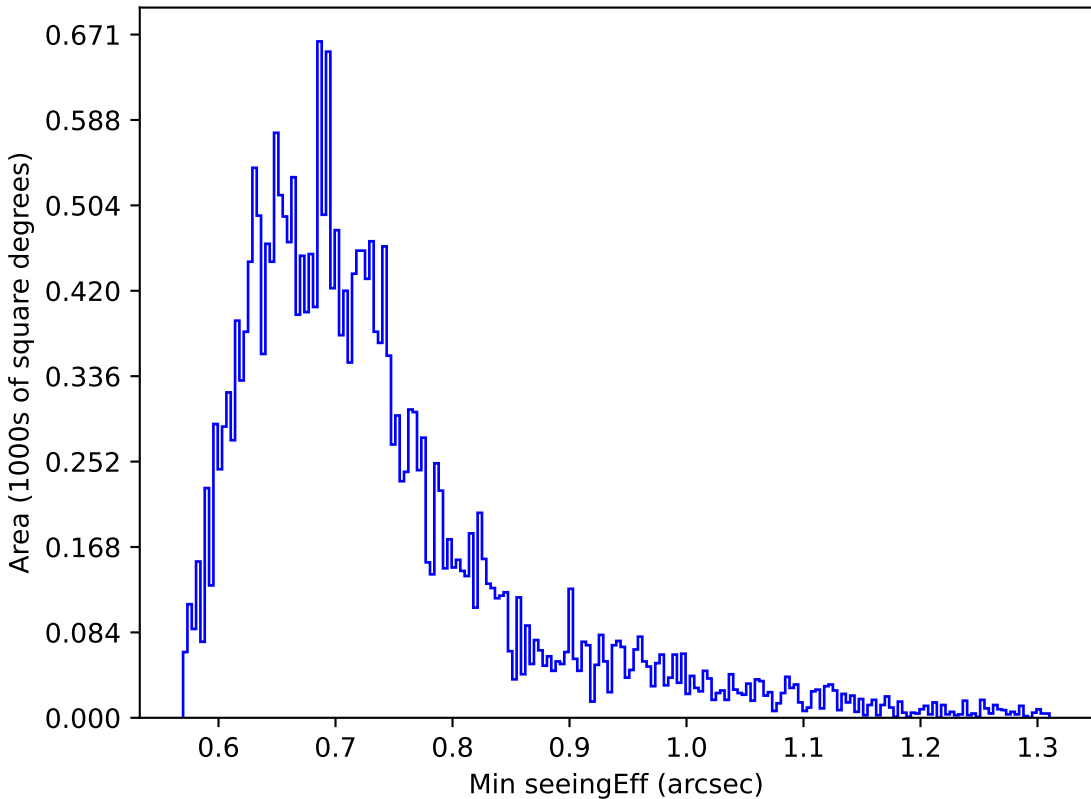
ddf_acor_sf25_lsf30_lsr10_v3.4_10yrs Yr 1 z band: Min seeingEff
