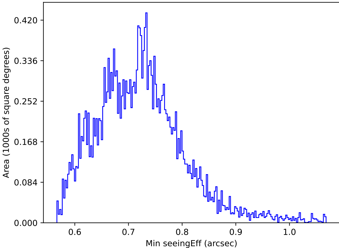
ddf_acor_sf25_lsf30_lsr10_v3.4_10yrs Yr 1 y band: Min seeingEff
