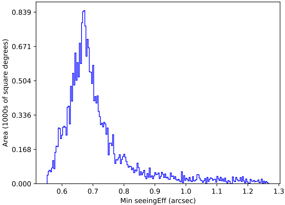
ddf_acor_sf25_lsf30_lsr10_v3.4_10yrs Yr 1 i band: Min seeingEff
