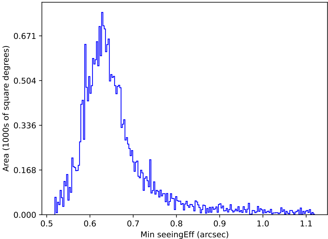
ddf_acor_sf25_lsf30_lsr10_v3.4_10yrs Yr 1 all bands: Min seeingEff
