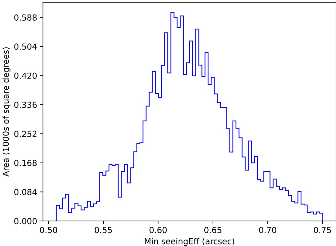
ddf_acor_sf25_lsf30_lsr10_v3.4_10yrs WFD y band: Min seeingEff
