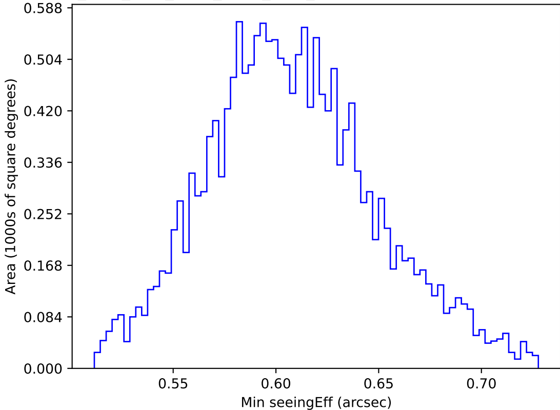
ddf_acor_sf25_lsf30_lsr10_v3.4_10yrs WFD i band: Min seeingEff
