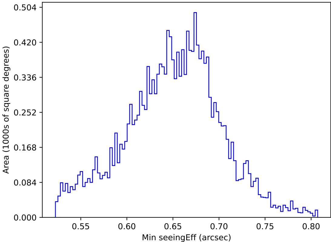
ddf_acor_sf25_lsf30_lsr10_v3.4_10yrs WFD g band: Min seeingEff
