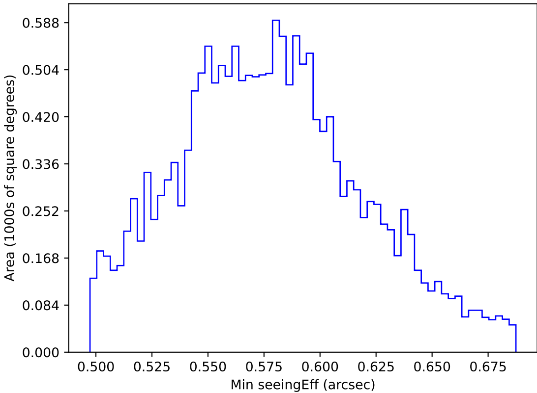
ddf_acor_sf25_lsf30_lsr10_v3.4_10yrs WFD all bands: Min seeingEff
