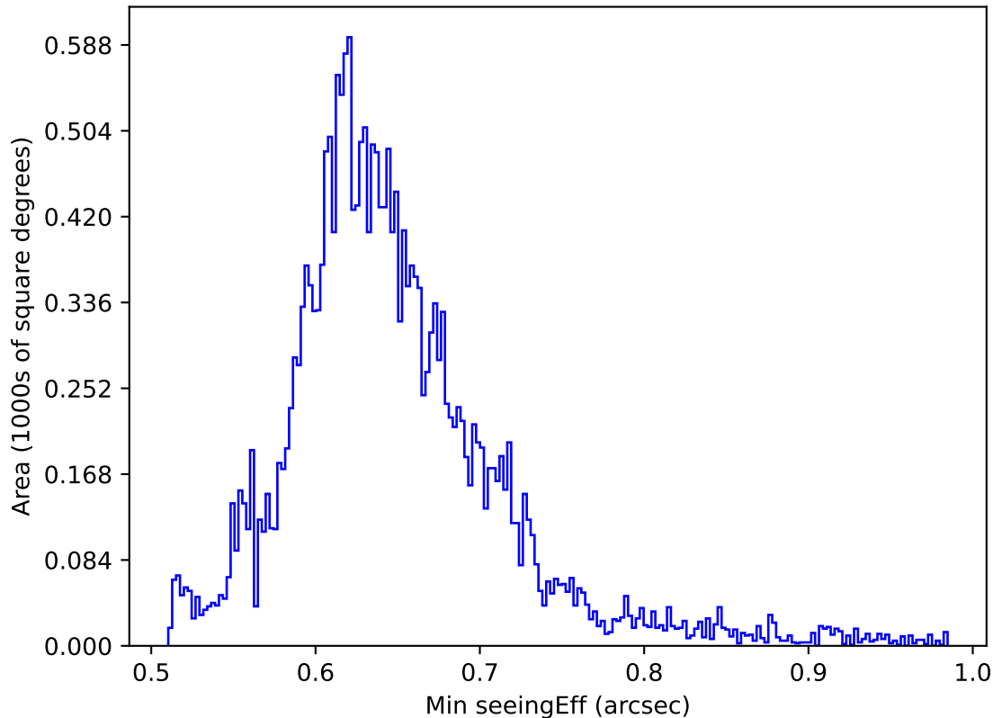
ddf_acor_sf25_lsf30_lsr10_v3.4_10yrs All sky y band: Min seeingEff
