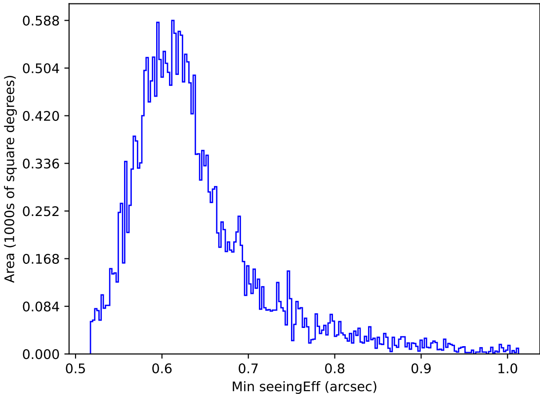
ddf_acor_sf25_lsf30_lsr10_v3.4_10yrs All sky i band: Min seeingEff
