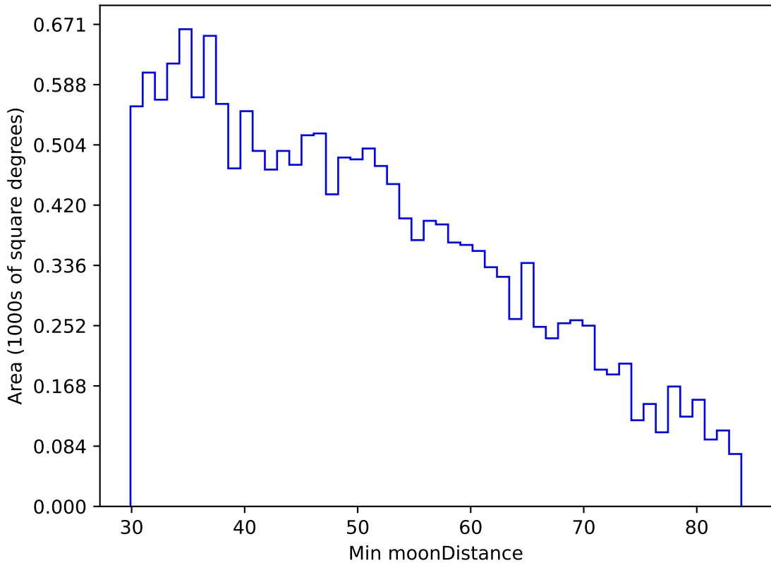
ddf_acor_sf25_lsf30_lsr10_v3.4_10yrs WFD u band: Min moonDistance
