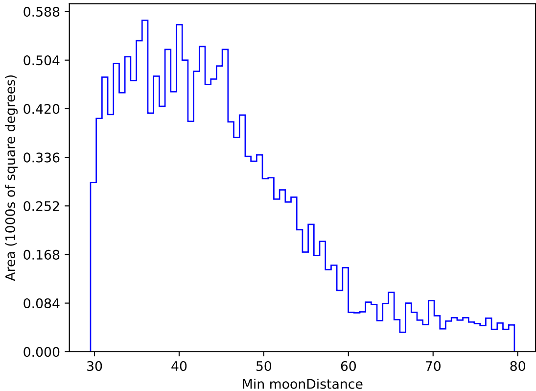
ddf_acor_sf25_lsf30_lsr10_v3.4_10yrs WFD g band: Min moonDistance
