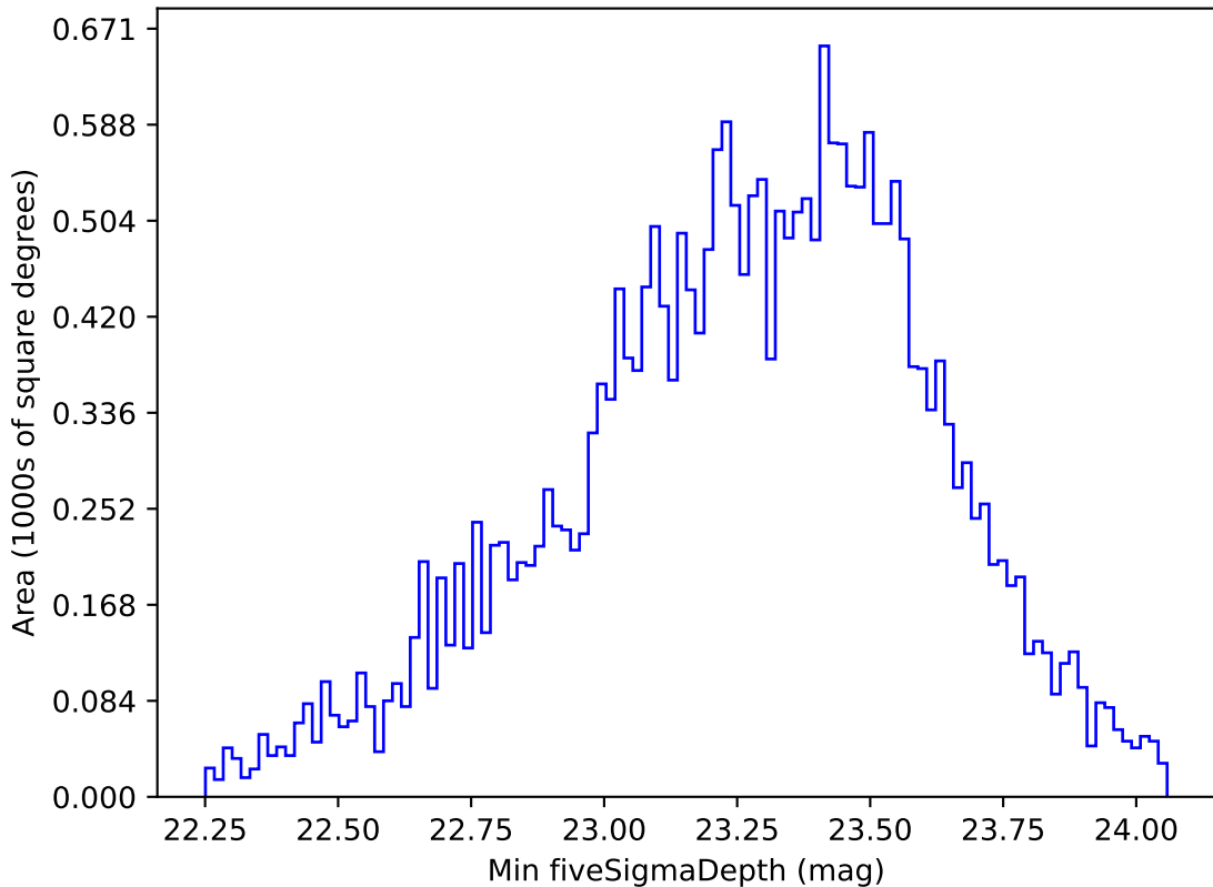
ddf_acor_sf25_lsf30_lsr10_v3.4_10yrs All sky g band: Min fiveSigmaDepth
