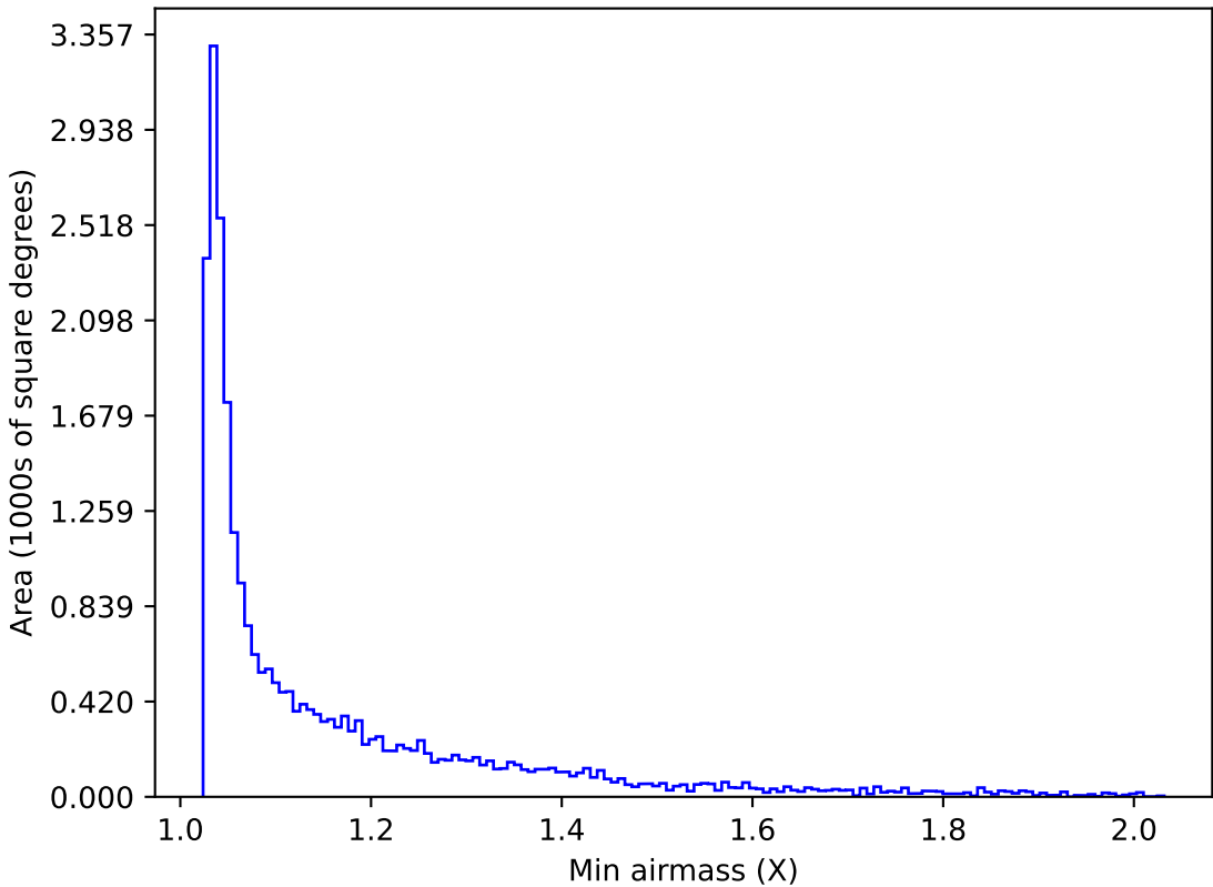
ddf_acor_sf25_lsf30_lsr10_v3.4_10yrs Yr 1 i band: Min airmass
