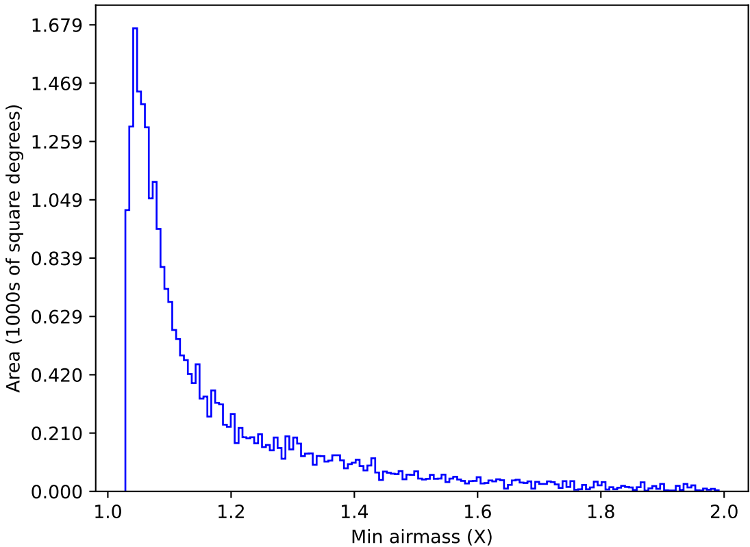
ddf_acor_sf25_lsf30_lsr10_v3.4_10yrs Yr 1 g band: Min airmass
