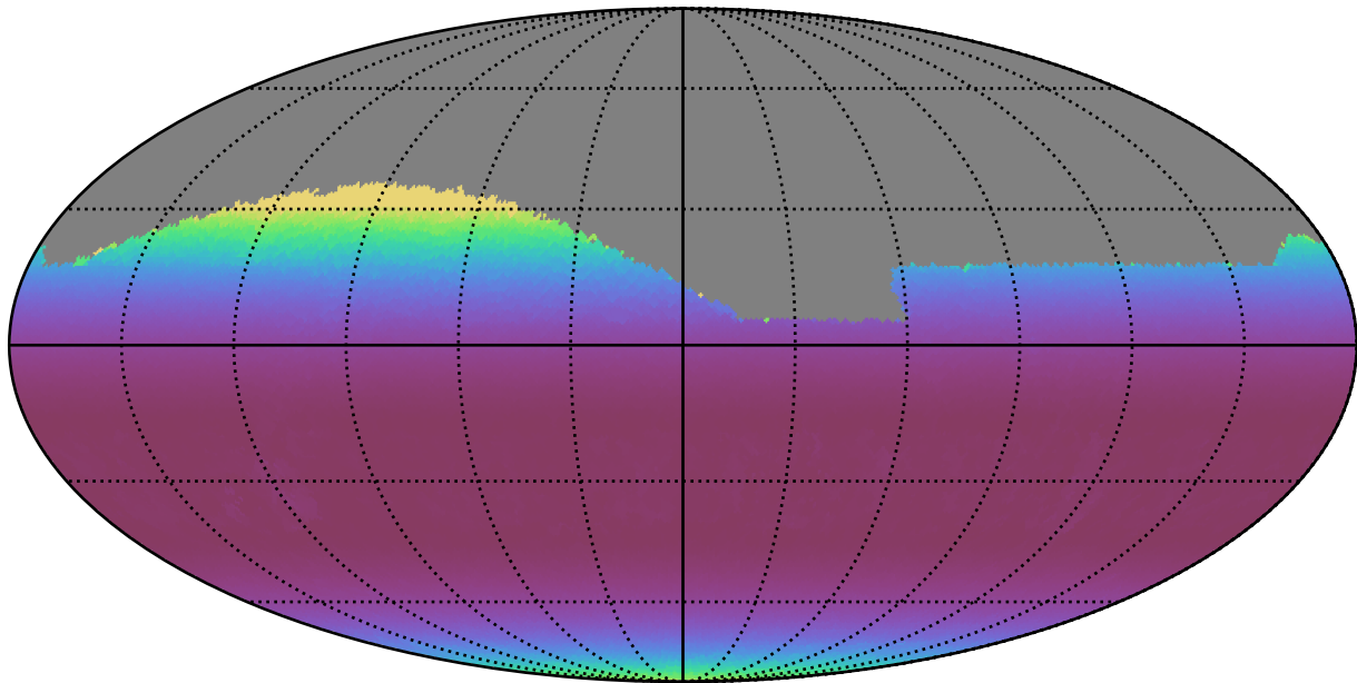
ddf_acor_sf25_lsf30_lsr10_v3.4_10yrs Yr 1 all bands: Min airmass
