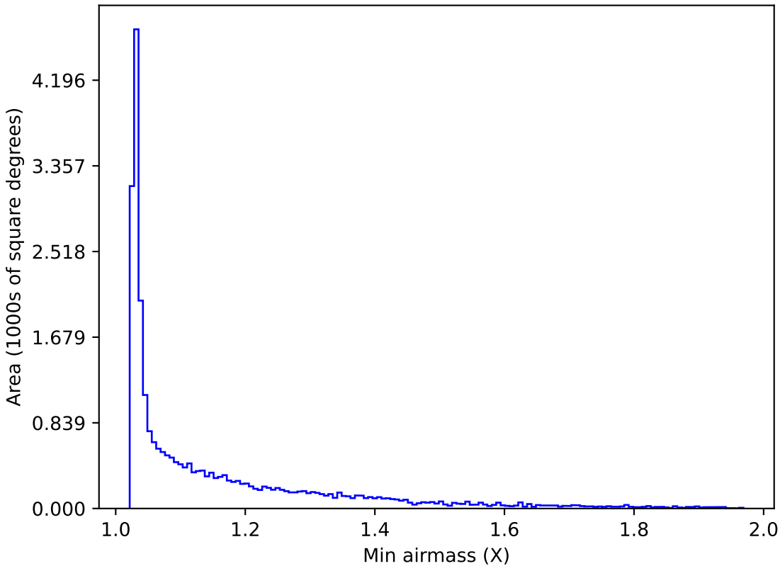
ddf_acor_sf25_lsf30_lsr10_v3.4_10yrs Yr 1 all bands: Min airmass
