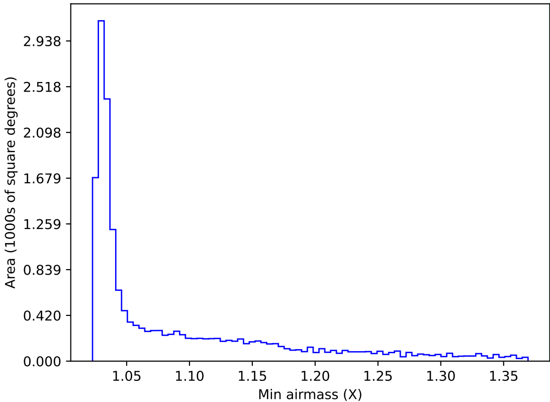
ddf_acor_sf25_lsf30_lsr10_v3.4_10yrs WFD y band: Min airmass
