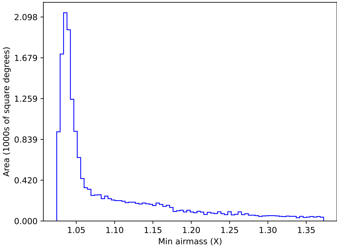
ddf_acor_sf25_lsf30_lsr10_v3.4_10yrs WFD u band: Min airmass
