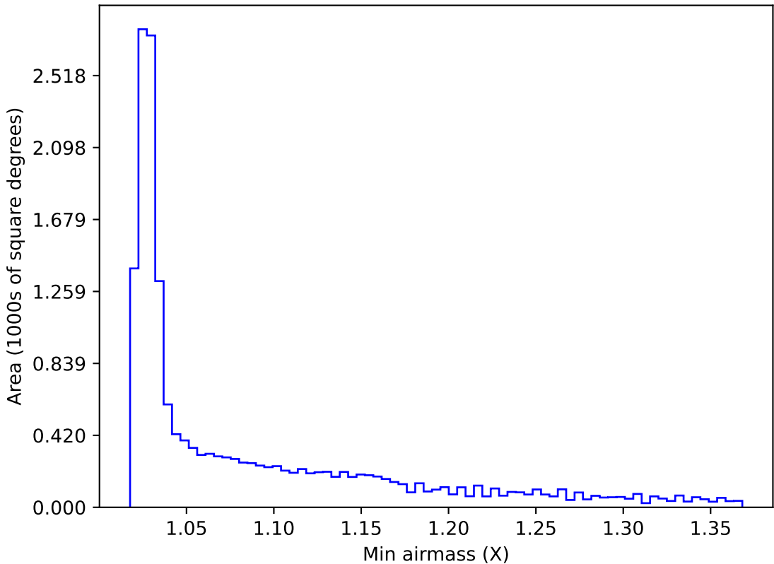
ddf_acor_sf25_lsf30_lsr10_v3.4_10yrs WFD r band: Min airmass
