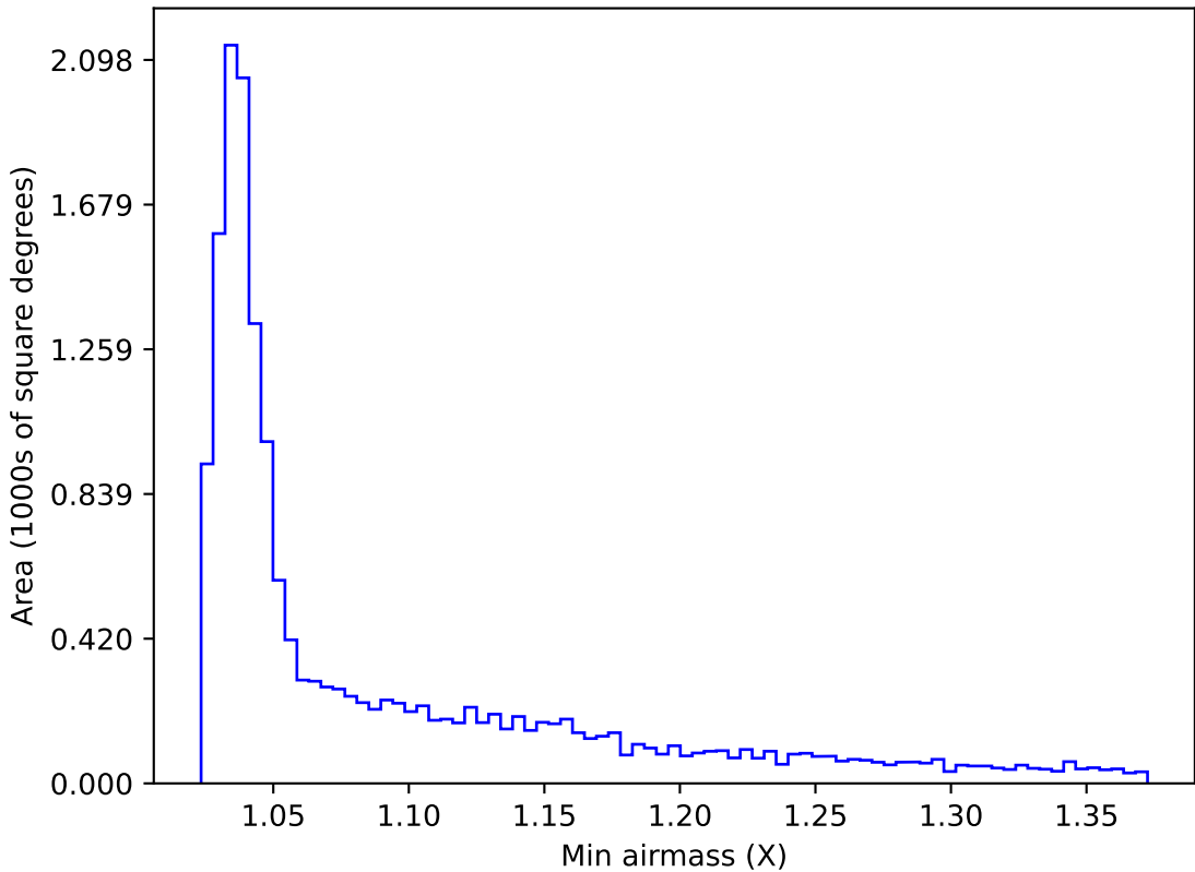
ddf_acor_sf25_lsf30_lsr10_v3.4_10yrs WFD g band: Min airmass
