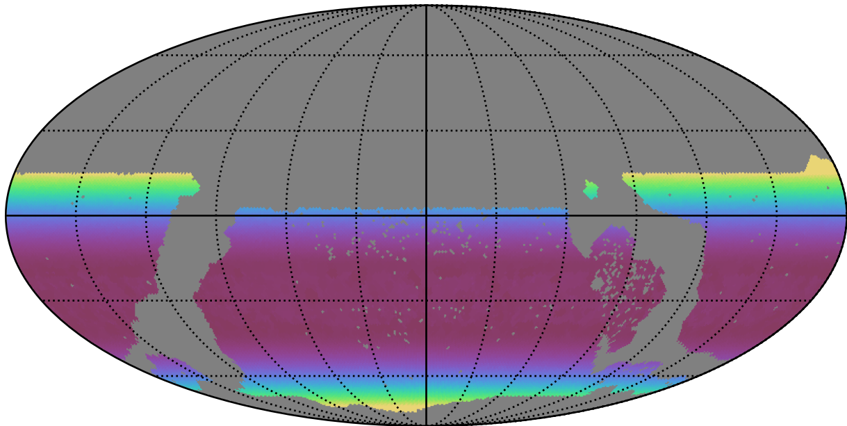
ddf_acor_sf25_lsf30_lsr10_v3.4_10yrs WFD all bands: Min airmass
