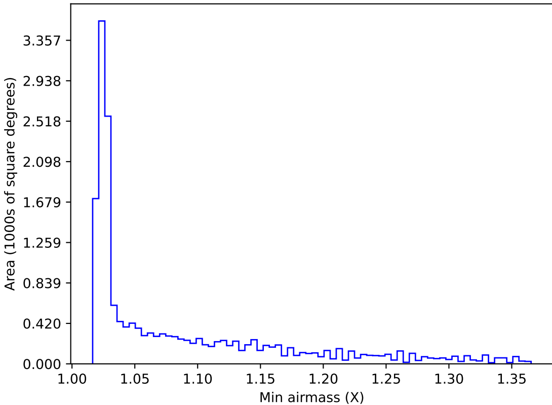
ddf_acor_sf25_lsf30_lsr10_v3.4_10yrs WFD all bands: Min airmass
