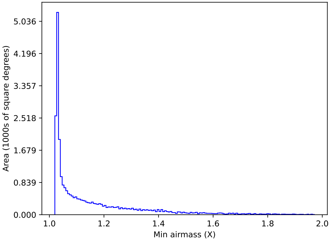
ddf_acor_sf25_lsf30_lsr10_v3.4_10yrs All sky z band: Min airmass
