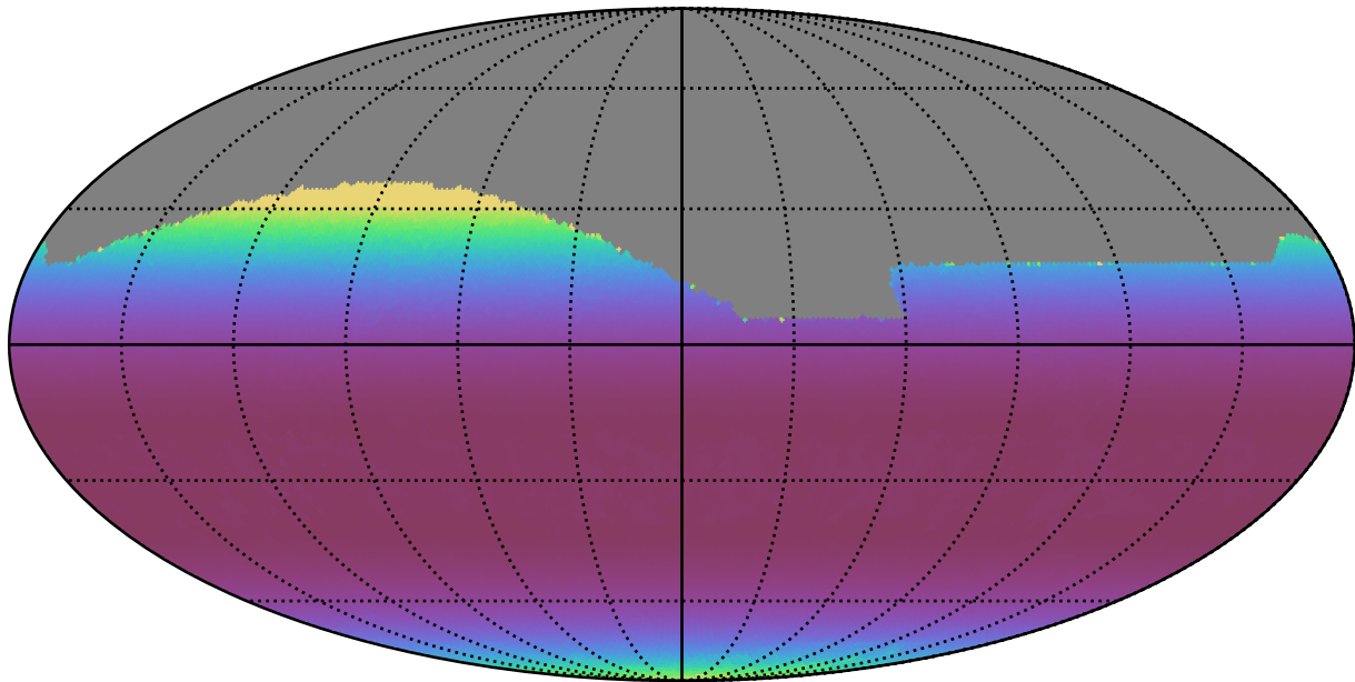
ddf_acor_sf25_lsf30_lsr10_v3.4_10yrs All sky r band: Min airmass
