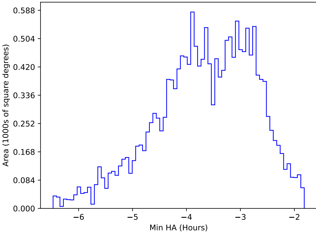
ddf_acor_sf25_lsf30_lsr10_v3.4_10yrs WFD y band: Min HA
