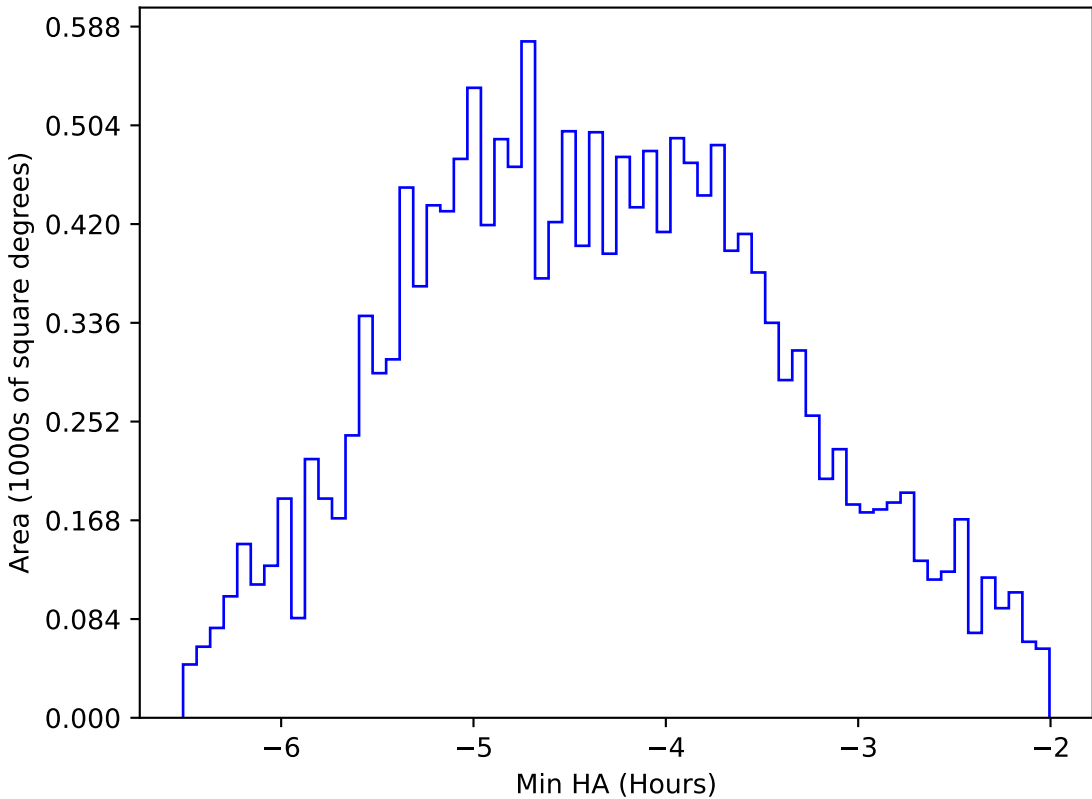
ddf_acor_sf25_lsf30_lsr10_v3.4_10yrs WFD i band: Min HA
