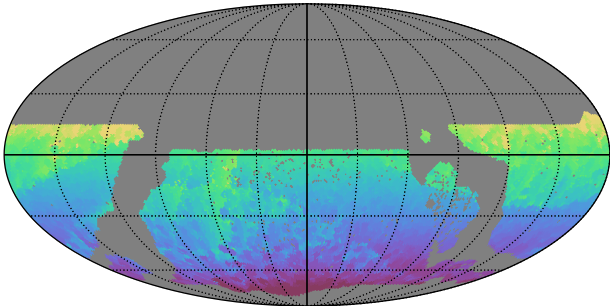
ddf_acor_sf25_lsf30_lsr10_v3.4_10yrs WFD all bands: Min HA
