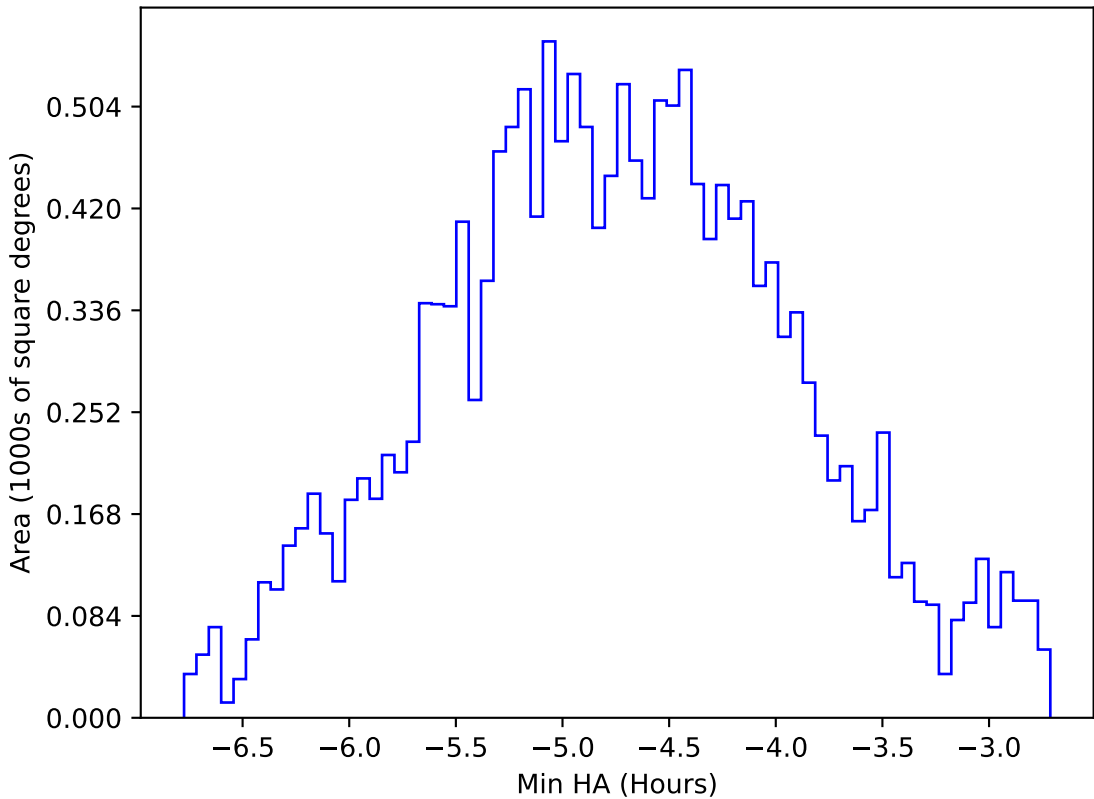
ddf_acor_sf25_lsf30_lsr10_v3.4_10yrs WFD all bands: Min HA
