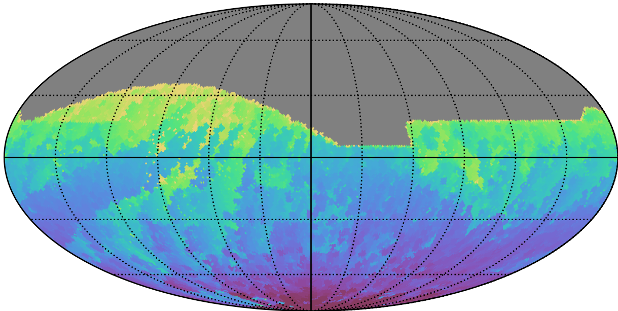
ddf_acor_sf25_lsf30_lsr10_v3.4_10yrs All sky z band: Min HA
