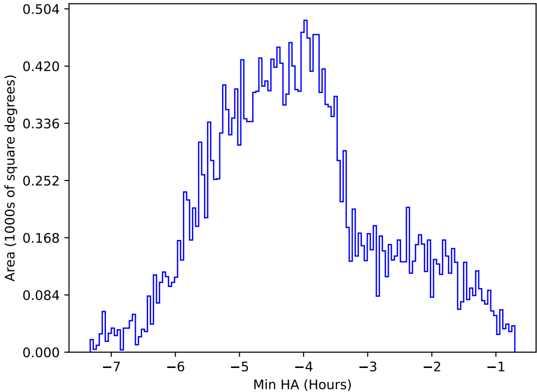
ddf_acor_sf25_lsf30_lsr10_v3.4_10yrs All sky z band: Min HA
