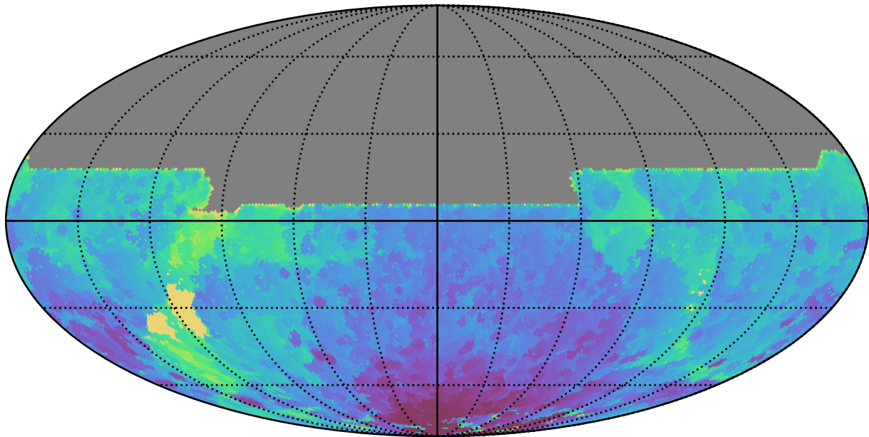
ddf_acor_sf25_lsf30_lsr10_v3.4_10yrs All sky y band: Min HA
