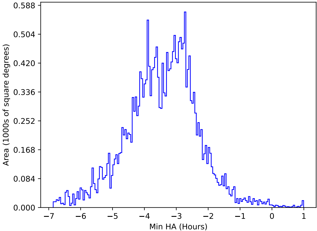
ddf_acor_sf25_lsf30_lsr10_v3.4_10yrs All sky y band: Min HA
