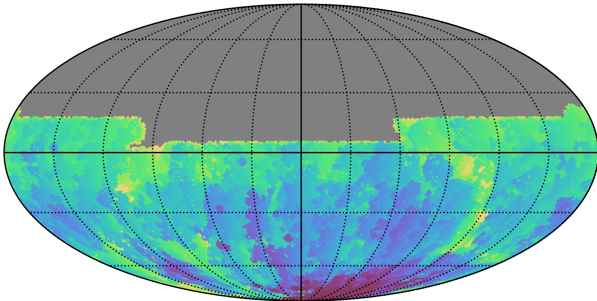
ddf_acor_sf25_lsf30_lsr10_v3.4_10yrs All sky u band: Min HA
