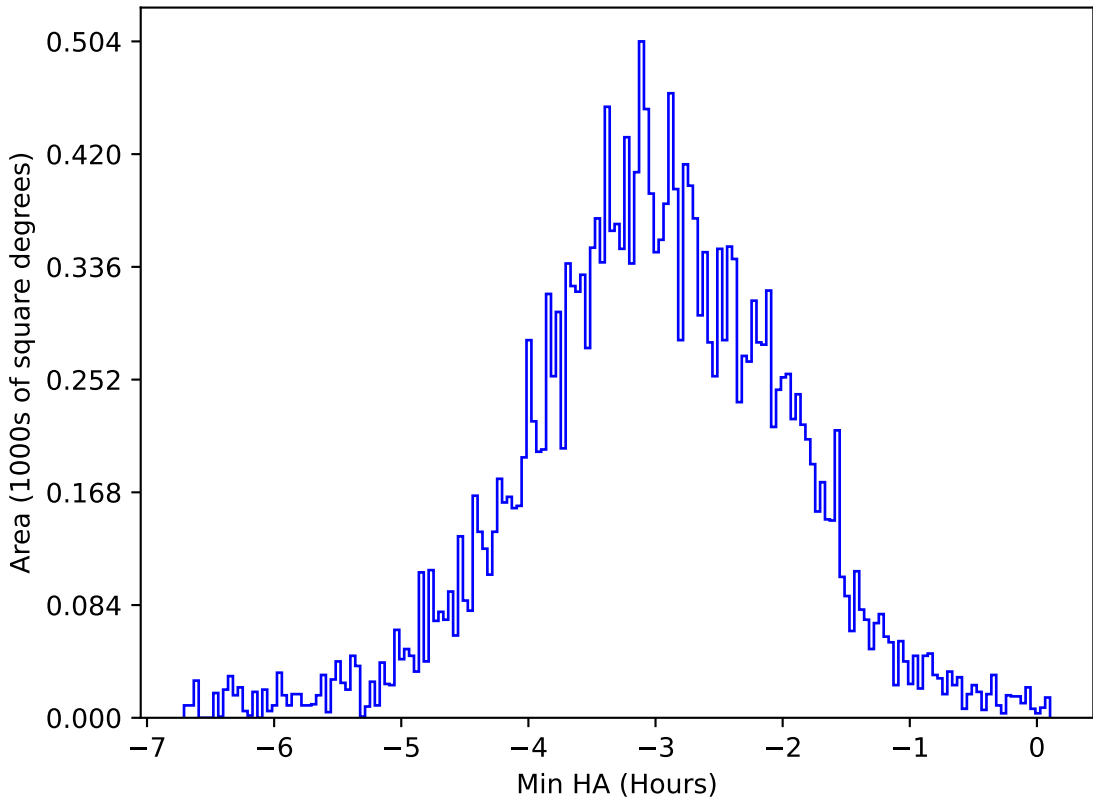
ddf_acor_sf25_lsf30_lsr10_v3.4_10yrs All sky u band: Min HA
