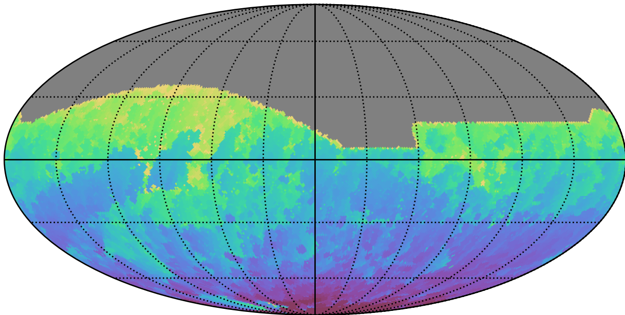
ddf_acor_sf25_lsf30_lsr10_v3.4_10yrs All sky i band: Min HA
