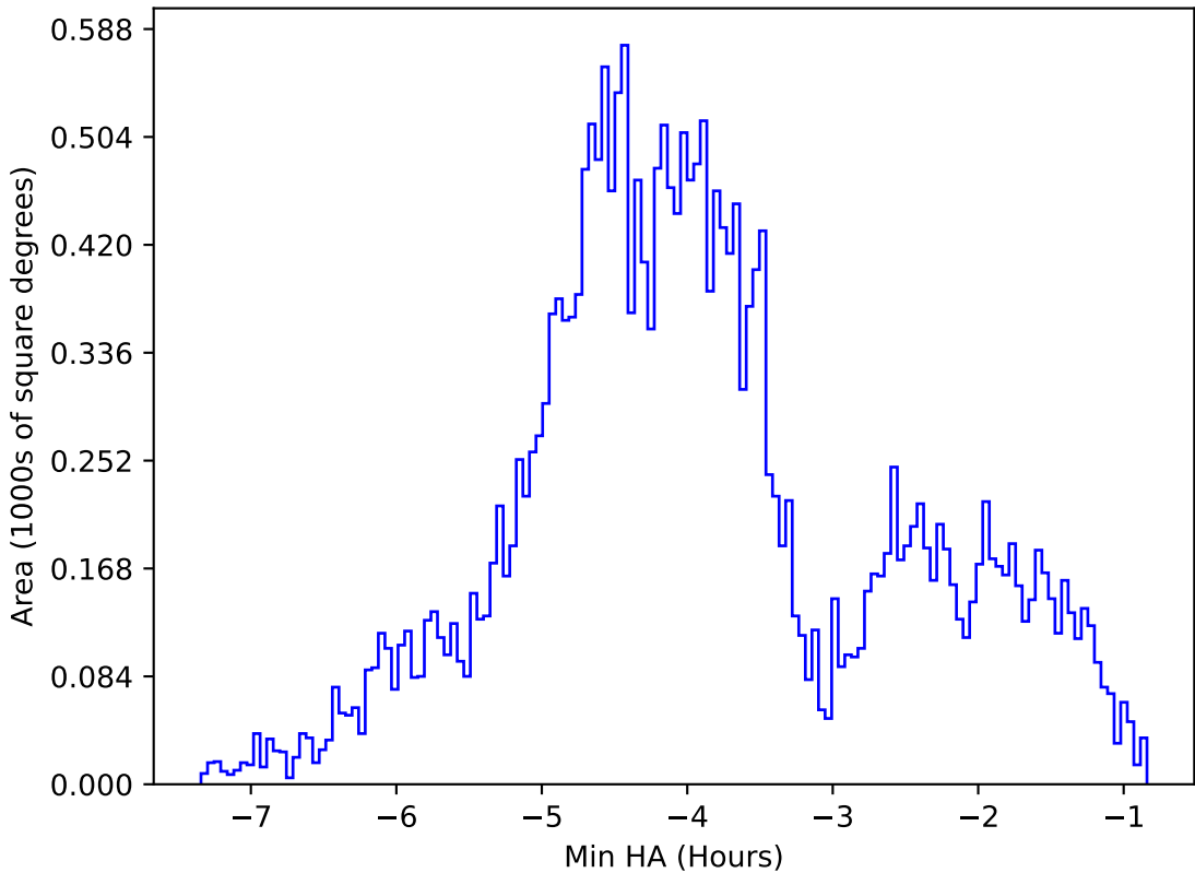
ddf_acor_sf25_lsf30_lsr10_v3.4_10yrs All sky g band: Min HA
