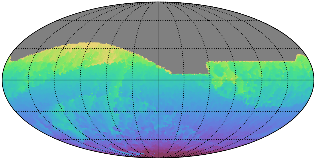
ddf_acor_sf25_lsf30_lsr10_v3.4_10yrs All sky all bands: Min HA
