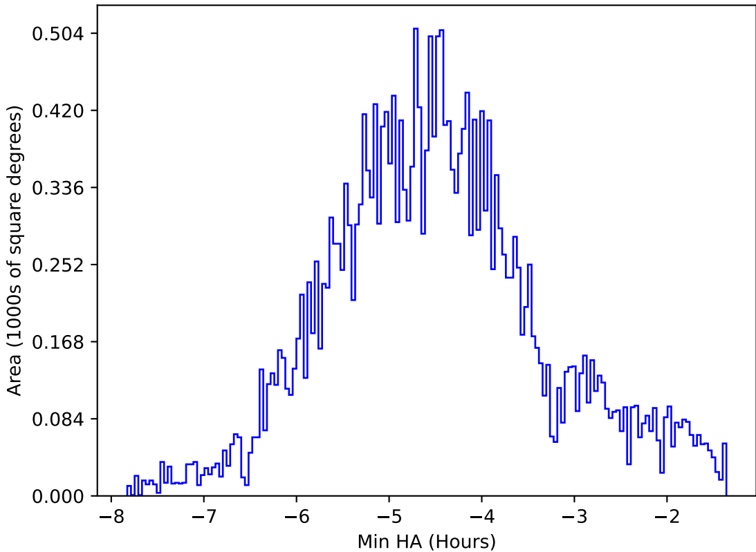
ddf_acor_sf25_lsf30_lsr10_v3.4_10yrs All sky all bands: Min HA
