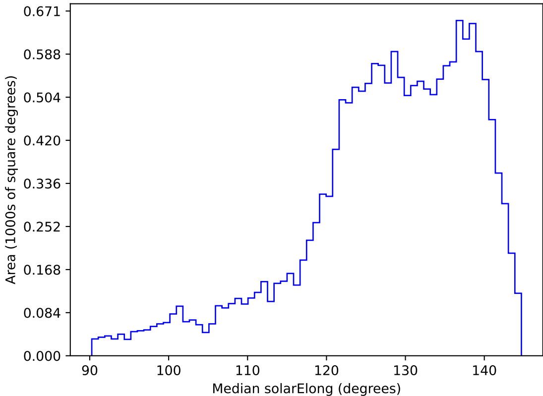
ddf_acor_sf25_lsf30_lsr10_v3.4_10yrs WFD z band: Median solarElong
