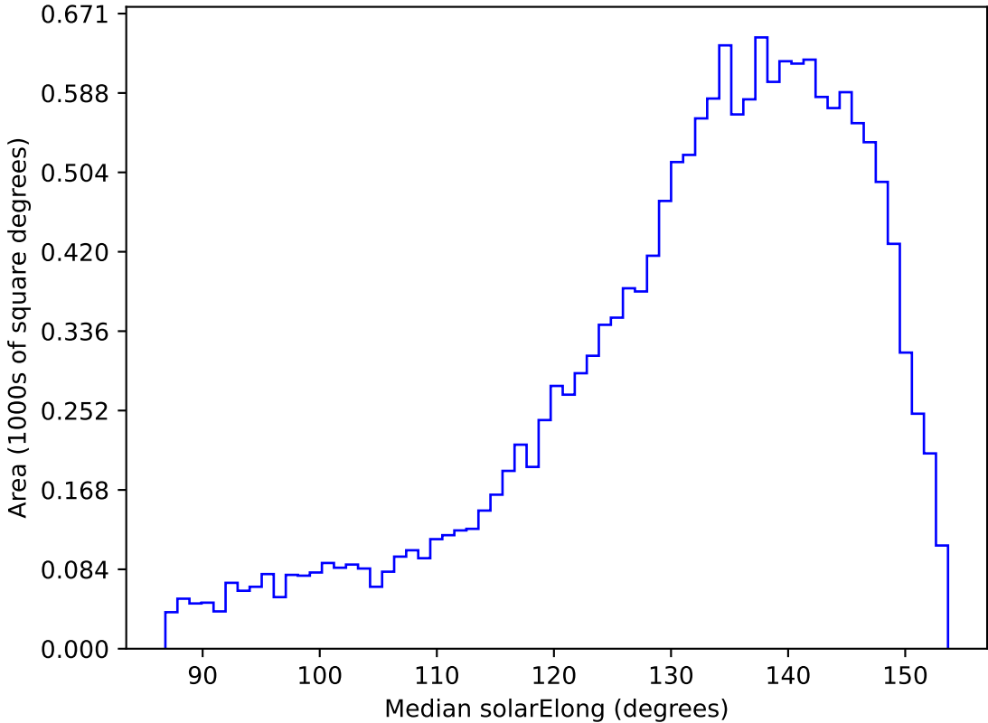
ddf_acor_sf25_lsf30_lsr10_v3.4_10yrs WFD u band: Median solarElong
