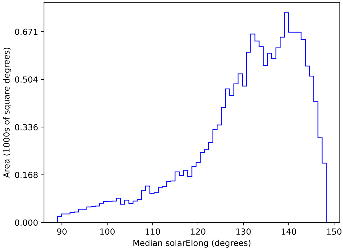
ddf_acor_sf25_lsf30_lsr10_v3.4_10yrs WFD r band: Median solarElong
