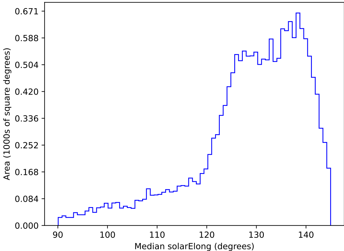
ddf_acor_sf25_lsf30_lsr10_v3.4_10yrs WFD i band: Median solarElong
