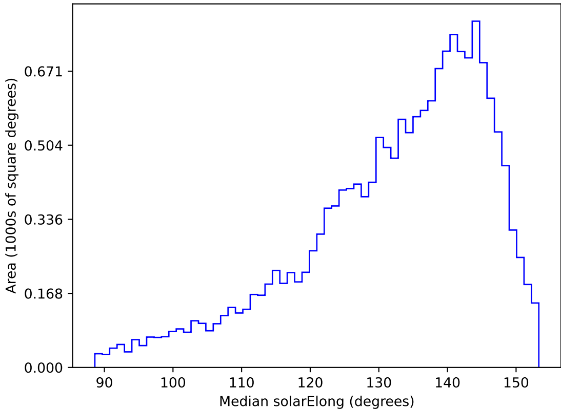
ddf_acor_sf25_lsf30_lsr10_v3.4_10yrs WFD g band: Median solarElong
