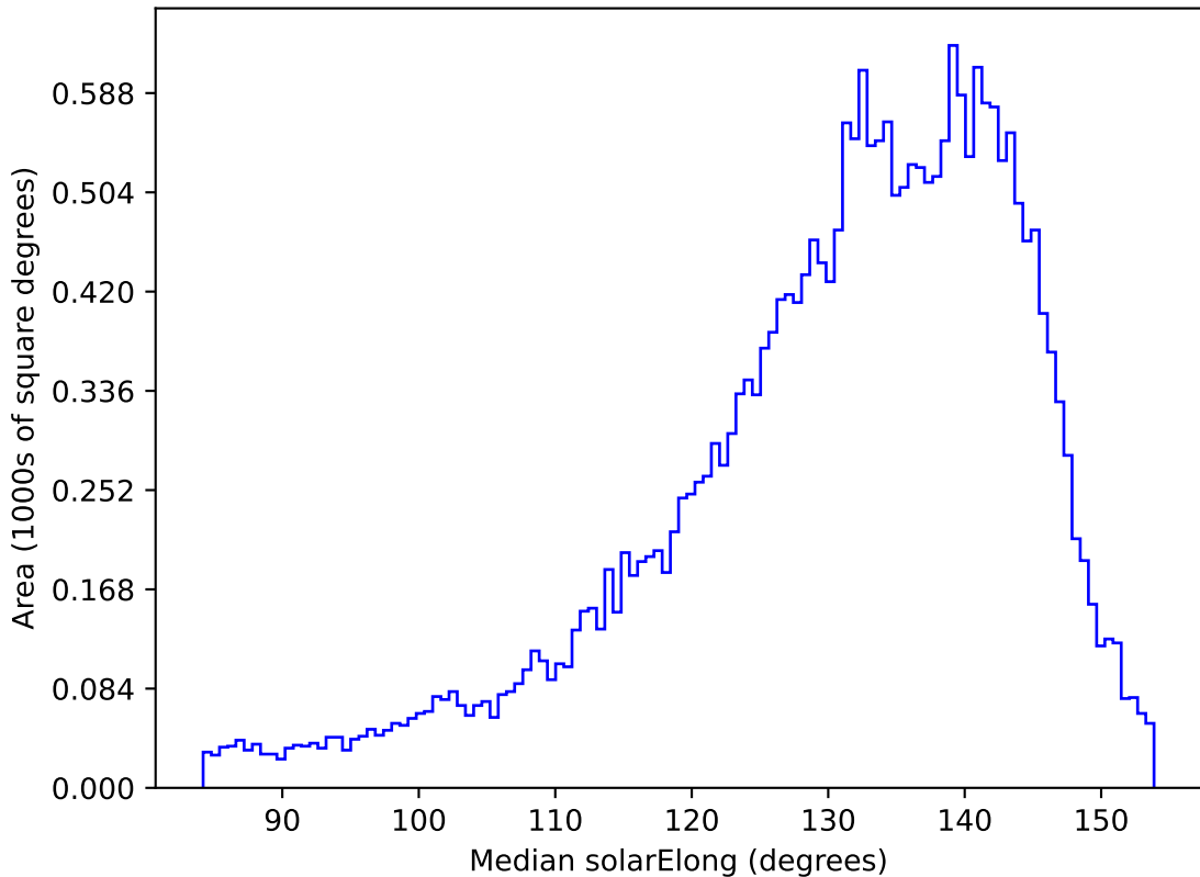
ddf_acor_sf25_lsf30_lsr10_v3.4_10yrs All sky r band: Median solarElong
