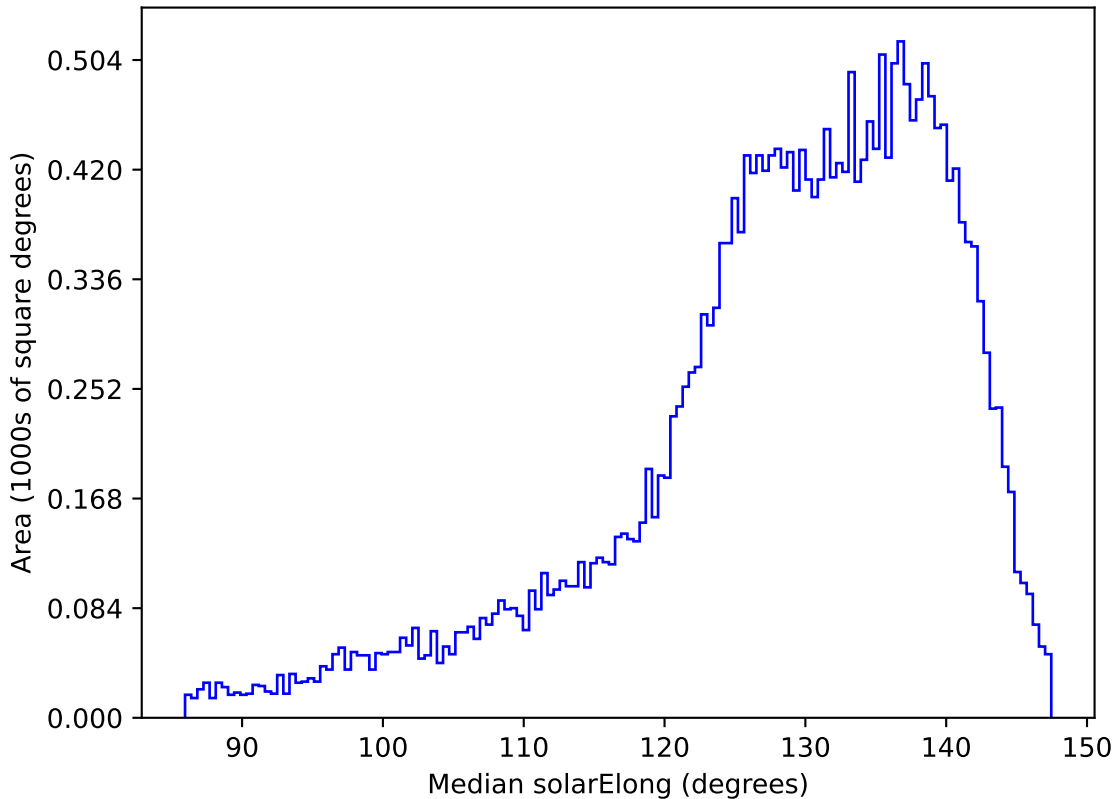
ddf_acor_sf25_lsf30_lsr10_v3.4_10yrs All sky i band: Median solarElong
