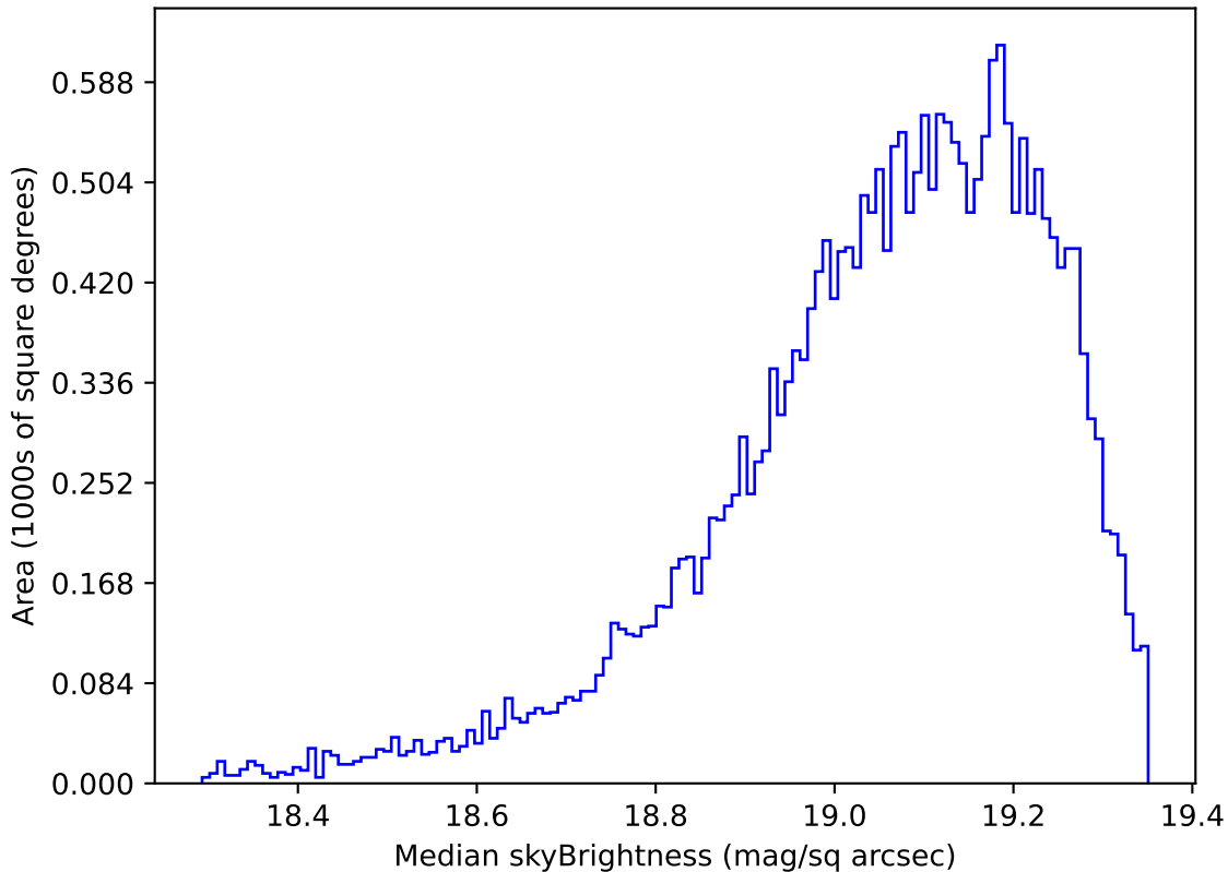
ddf_acor_sf25_lsf30_lsr10_v3.4_10yrs Yr 1 z band: Median skyBrightness
