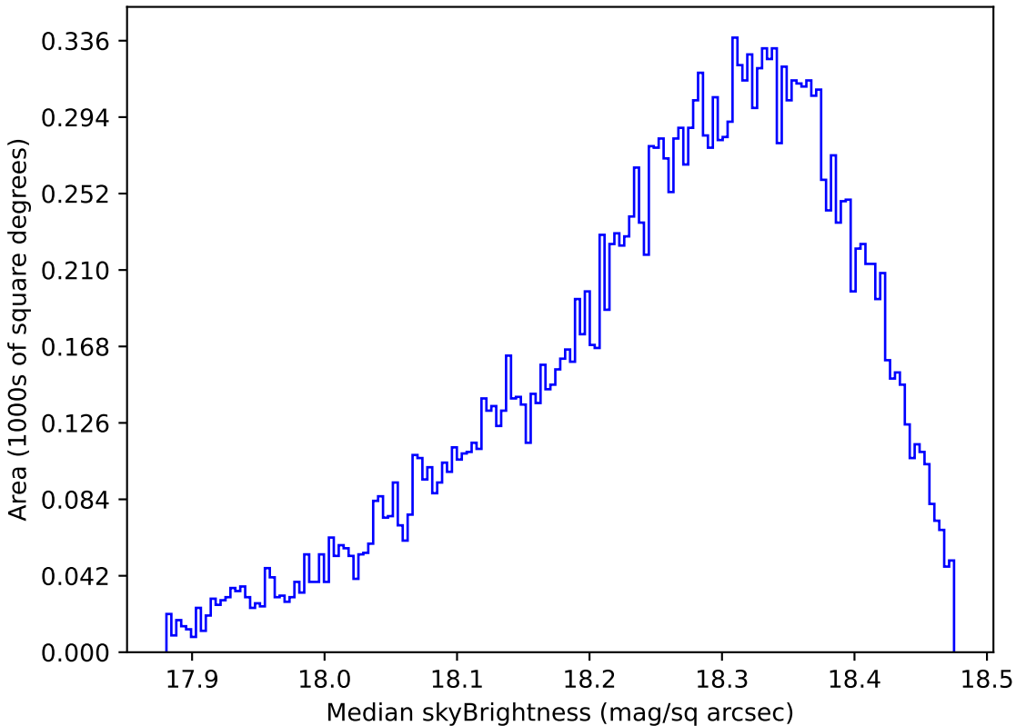
ddf_acor_sf25_lsf30_lsr10_v3.4_10yrs Yr 1 y band: Median skyBrightness
