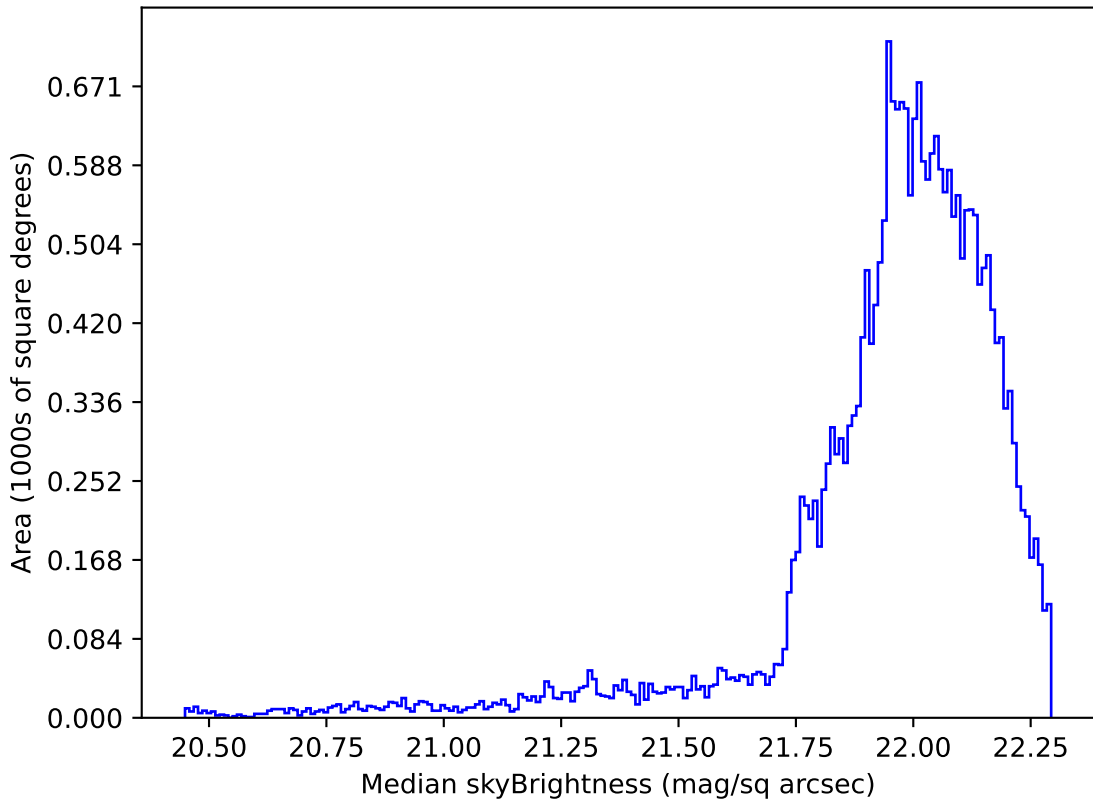
ddf_acor_sf25_lsf30_lsr10_v3.4_10yrs Yr 1 g band: Median skyBrightness
